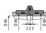
sectional detail pipe connection (without clamping ring)
